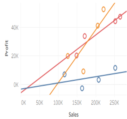
Scatter plot
