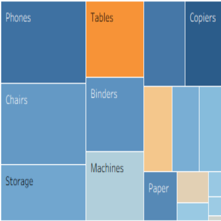
Tree Map
