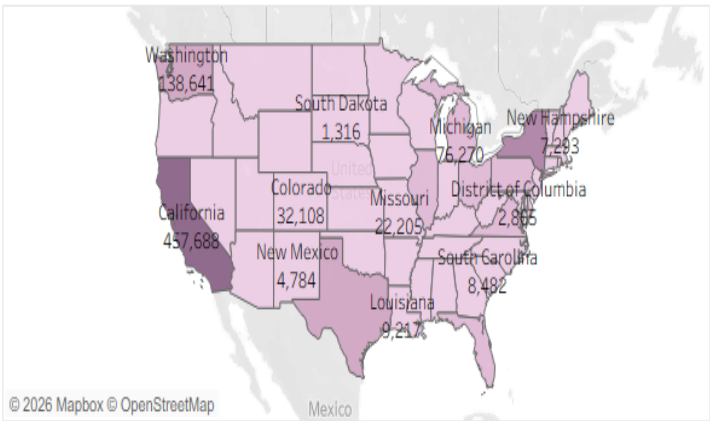
Map Chart
