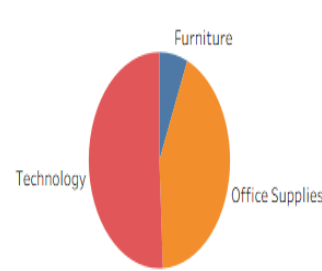
Pie Chart
